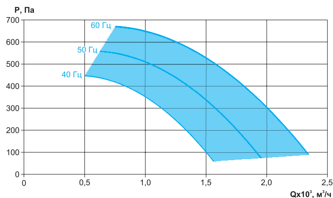
ВРС-К-60-35/25-РК635-0,37/3000/220-380
