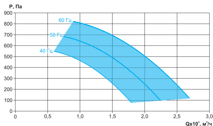
ВРС-К-60-30/25-РЦ-0,75/3000/220-380
