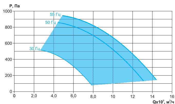
VCR-830/56-ПЦ-3,0/1500/220-380
